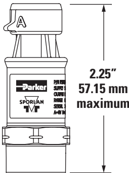
PRESSURE TRANSDUCER
